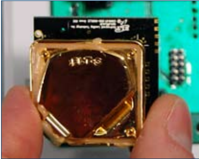
Field replaceable gold-plated CO2 NDIR
